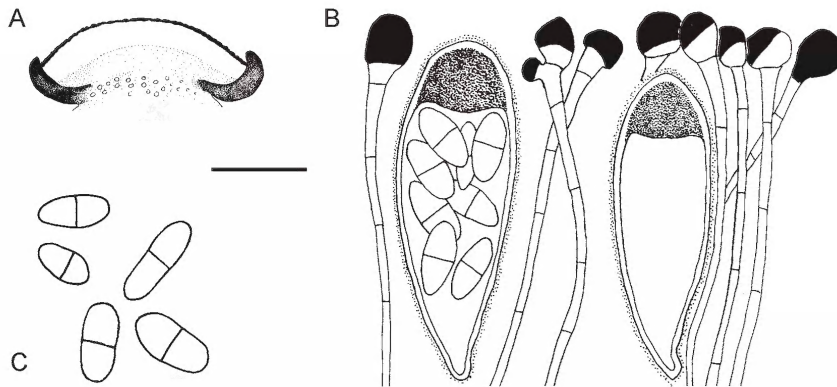
Fig. 2. Catillaria australittoralis (holotype): A vertical section of apothecium (schematic); B–C portion of hymenium and ascospores with amyloid tissues stippled. Scale bar: A 200 \mu m, B 10 \mu m.
